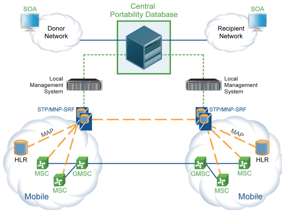
Number Portability Network Topology
